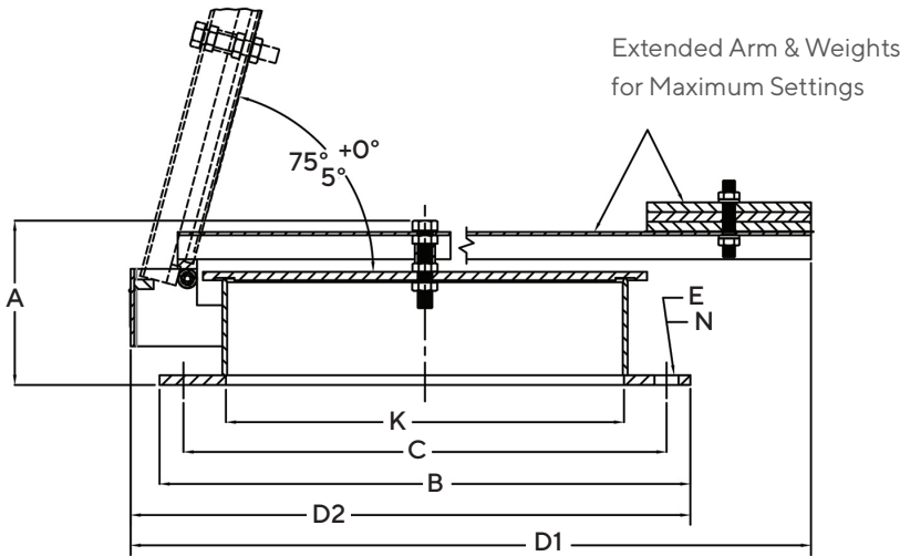
(Dimensions shown are for reference only, contact factory for certified drawings)
