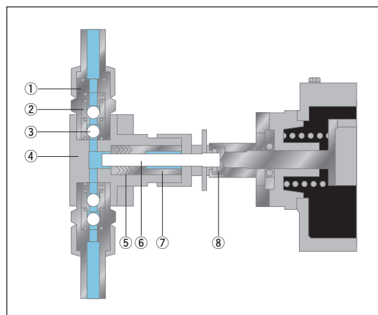
① Joint ② Valve seat ③ Check ball ④ Pump head ⑤ V-packing ⑥ Plunger ⑦ Packing retainer ⑧ Universal Joint
